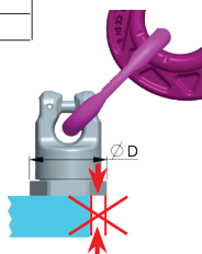
Pic. 2: Thread of the PP must be completely engaged and the lifting point must be installed full-faced. (The diameter of the bearing surface must be ≥ D)
