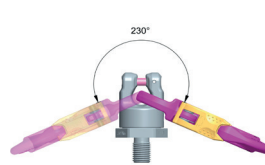
Pic. 4: Pivoting area of PP-S/PP-B/PP-VIP
